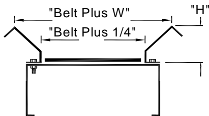
Flared Sides
