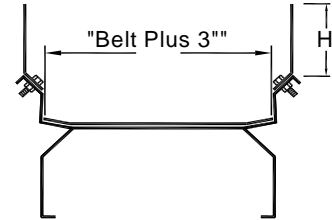
Trough Sides
