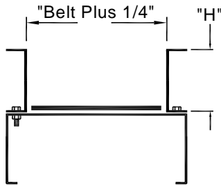
Channel Sides
